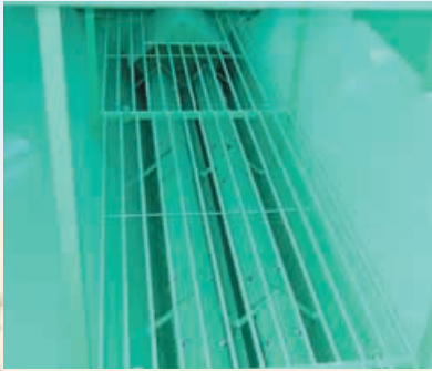
Large capacity hopper with floor augers
